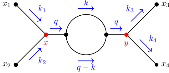
Figure 3.4: 1-loop correction of the s-channel diagram of the 2 \rightarrow 2 scattering process.
