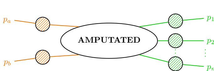
Figure 3.6: Structure of a fully interacting correlation function. To obtain the S-matrix element, the external legs containing the full propagator corrections (hatched circles) are amputated, leaving only the amputated connected Green's function in the center.
